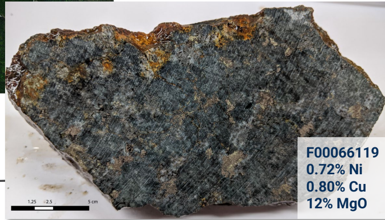
(1) E&L mineralized gabbro float collected W of Nickel Mountain
